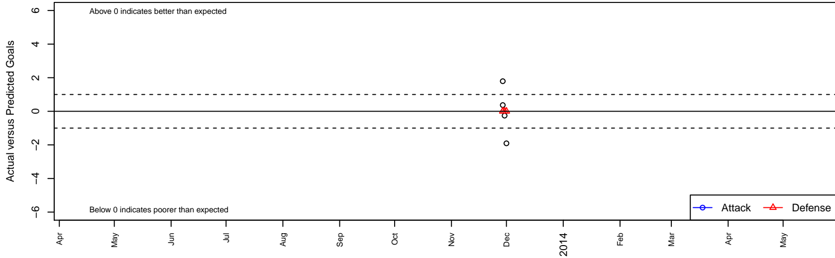
Alaska YS B97 Dots are actual minus expected GF (blue circles) and GA (red triangles). Blue line is smoothed change in attack strength. Red is smoothed change in defense strength.
